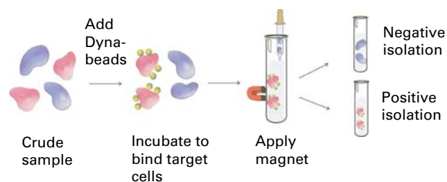
Figure 2 Immunomagnetic isolation.
